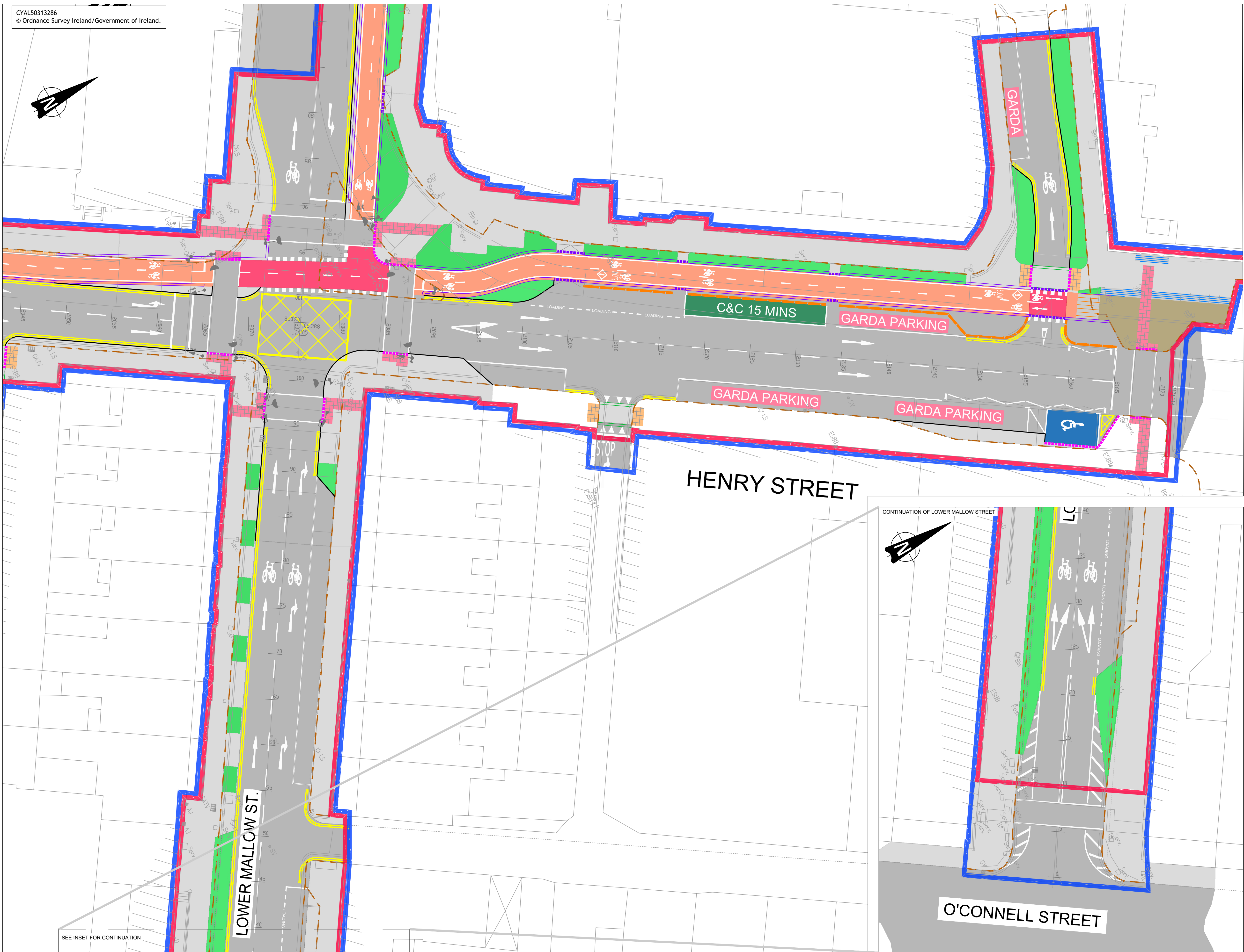
1:200 ROADS LAYOUT
