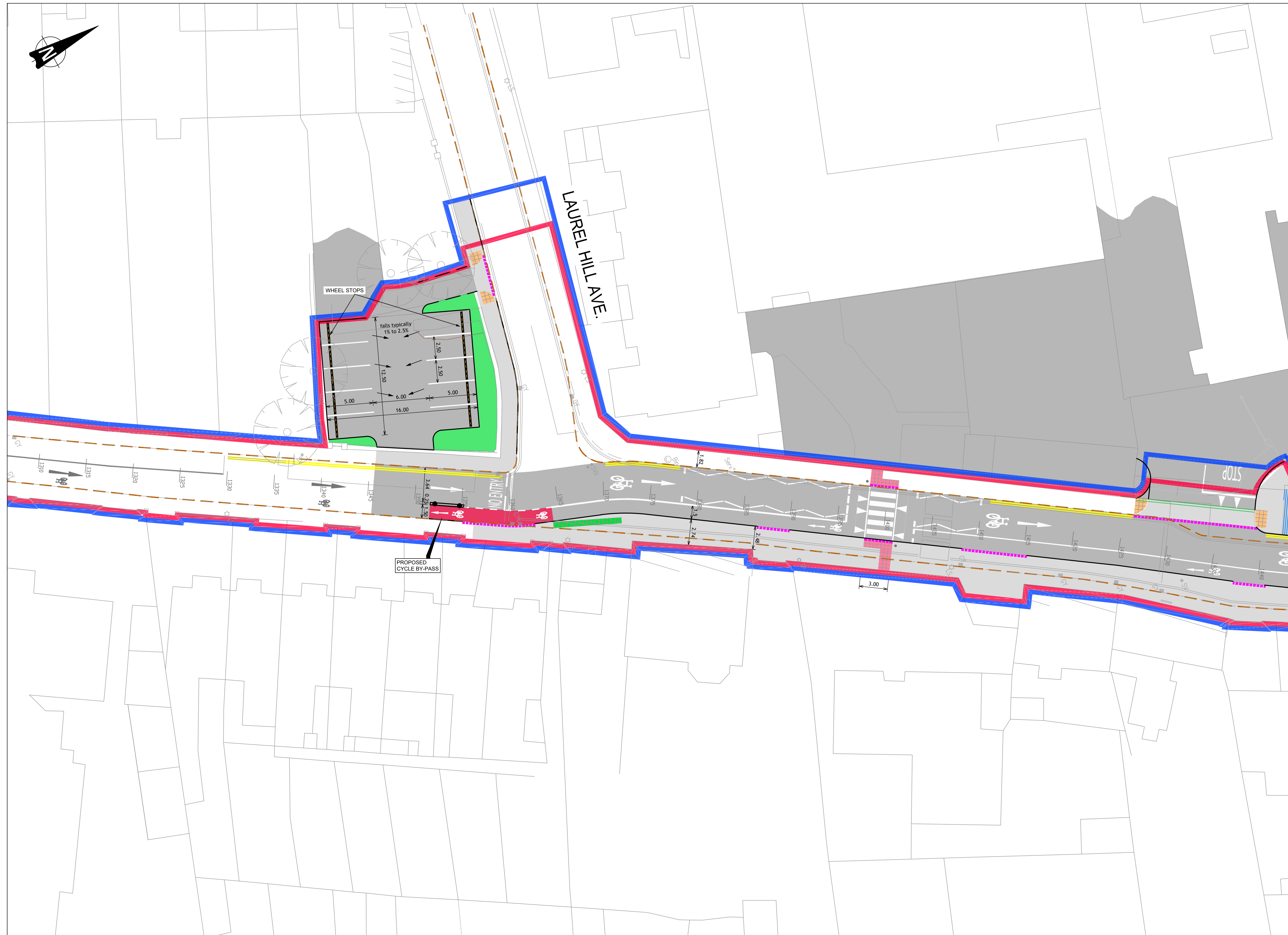
1:200 ROADS LAYOUT
