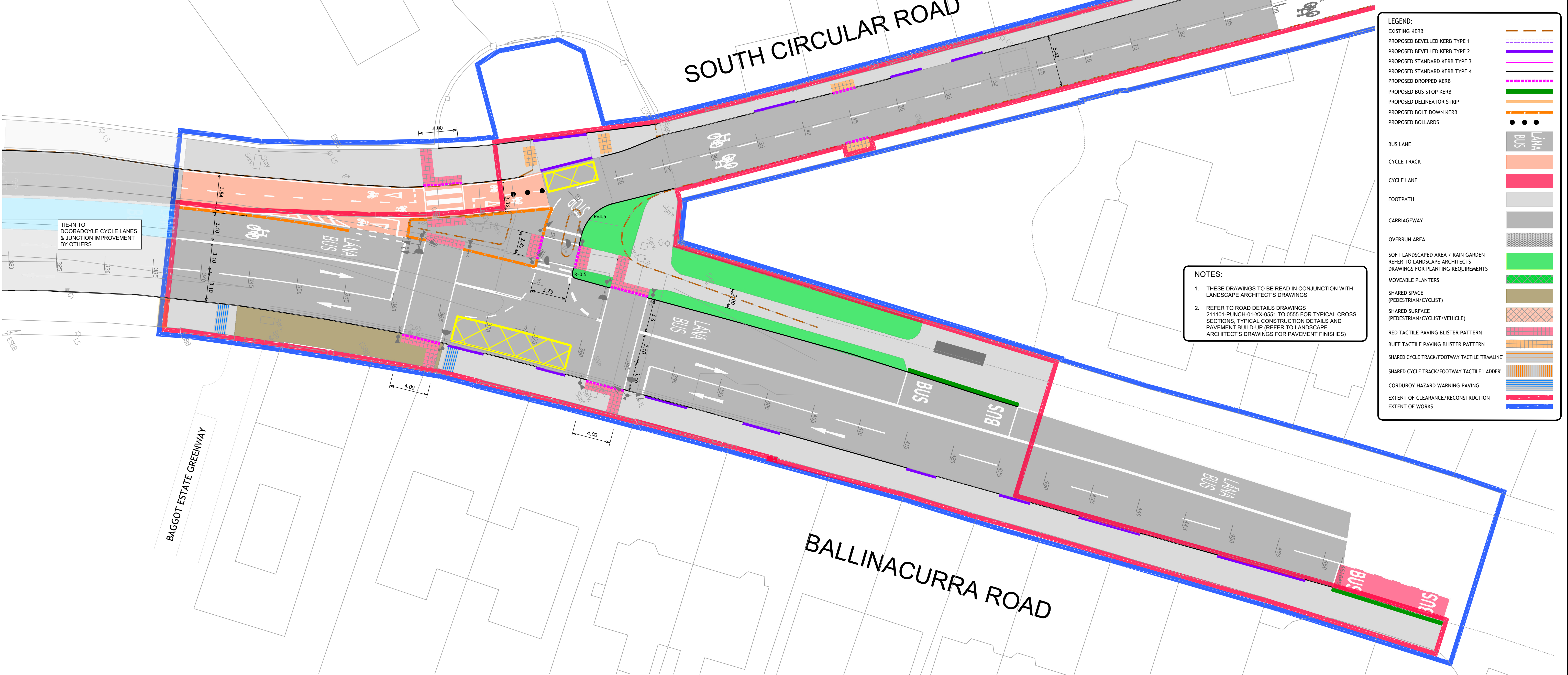
1:200 ROADS LAYOUT
