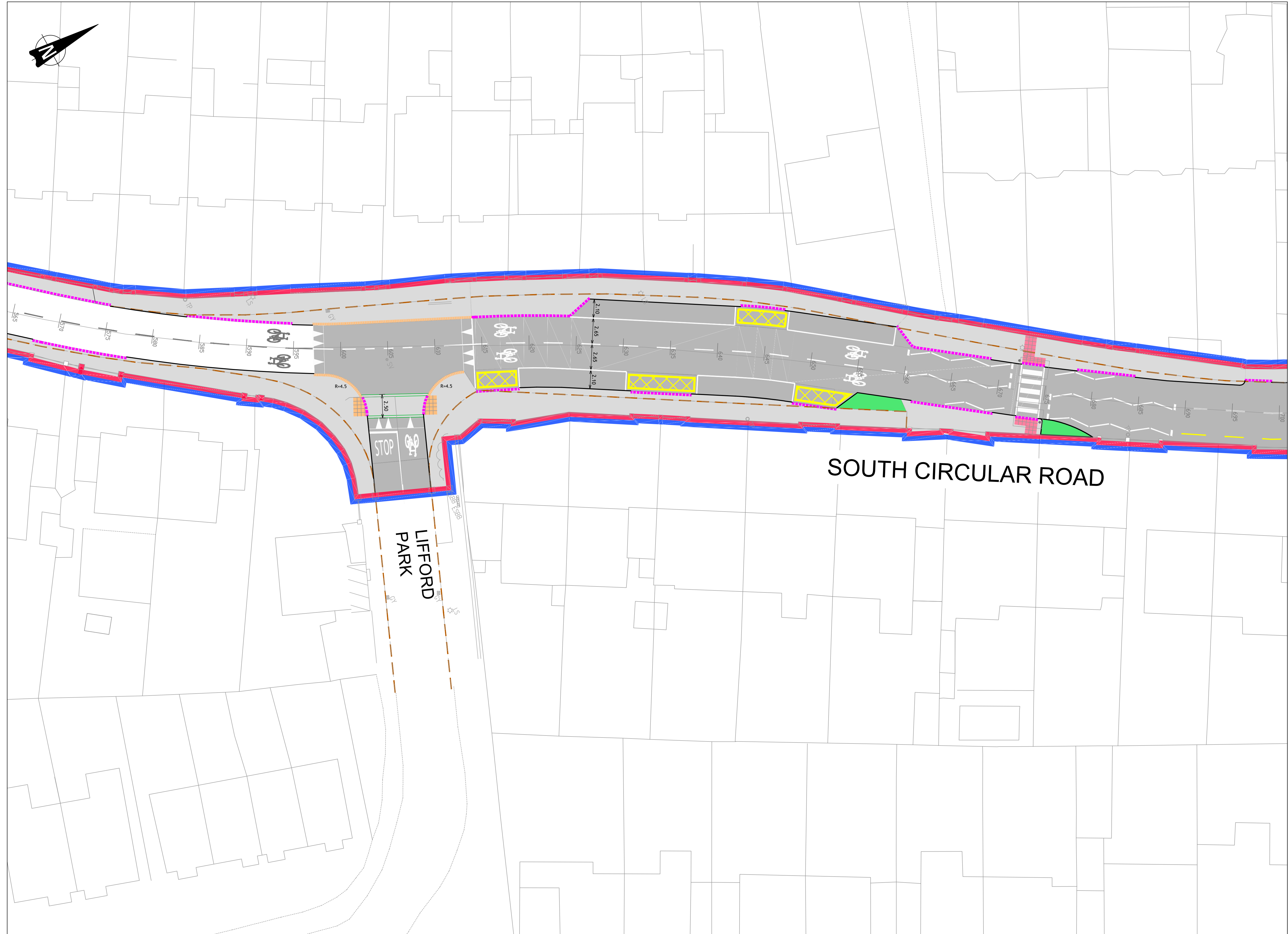
1:200 ROADS LAYOUT
