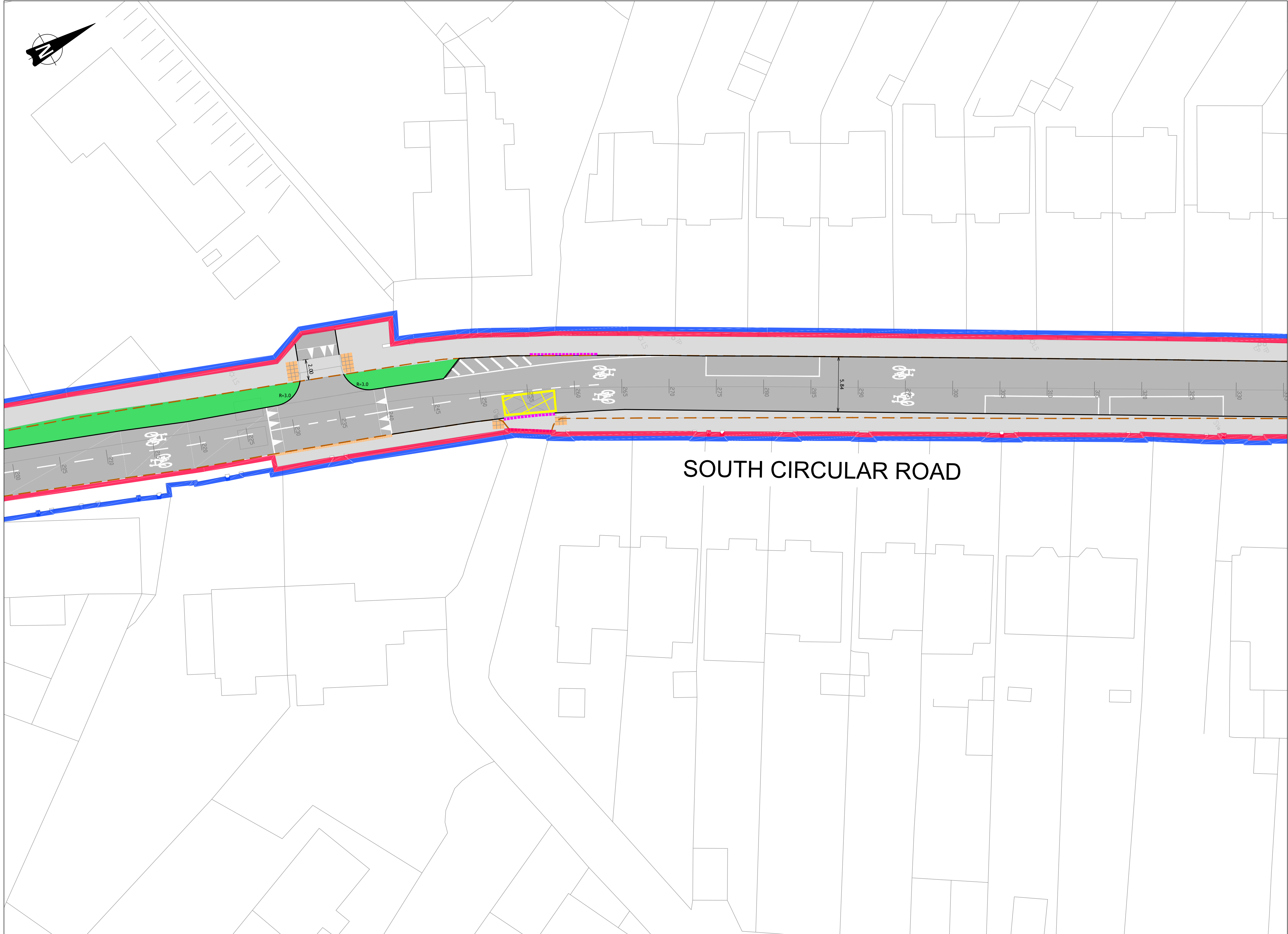
1:200 ROADS LAYOUT
