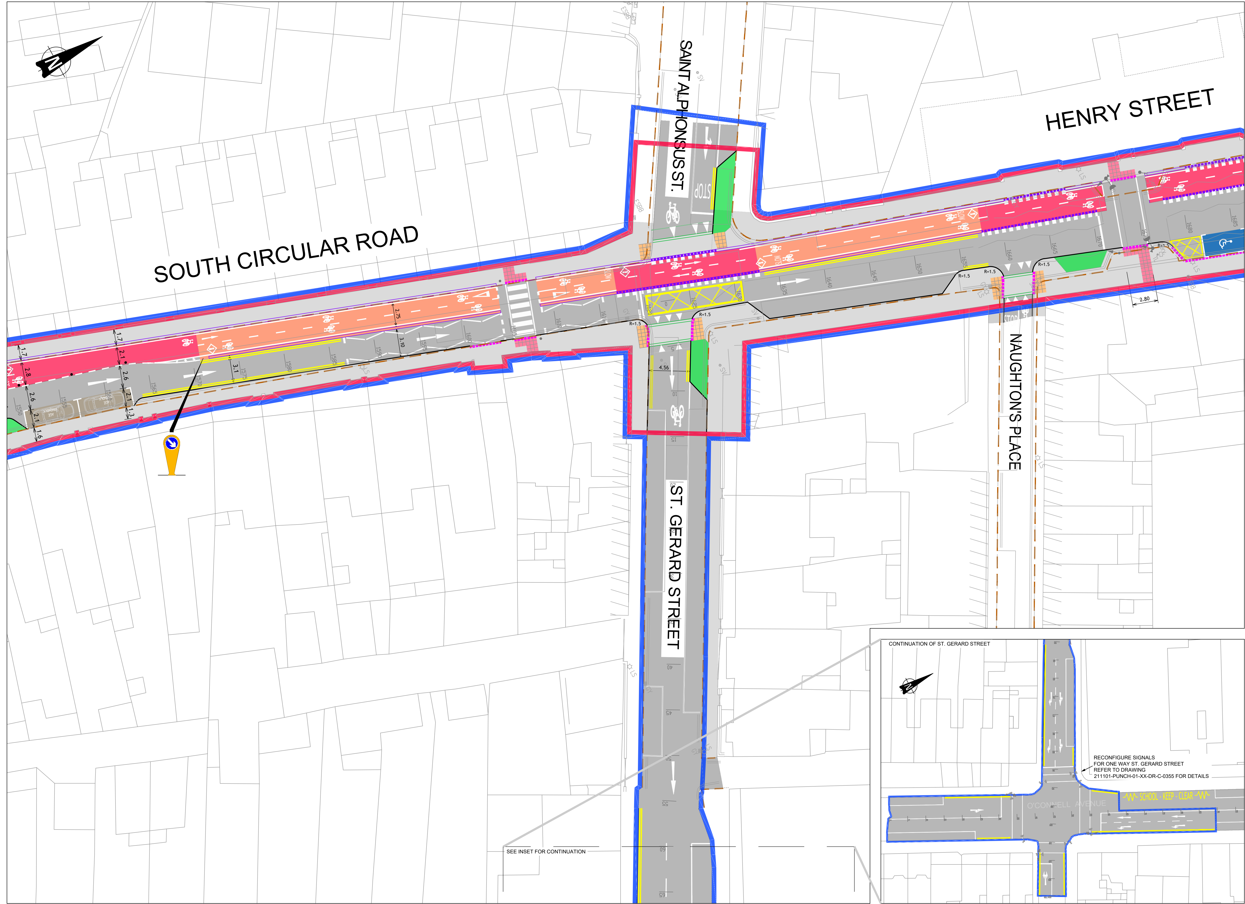
1:200 ROADS LAYOUT
