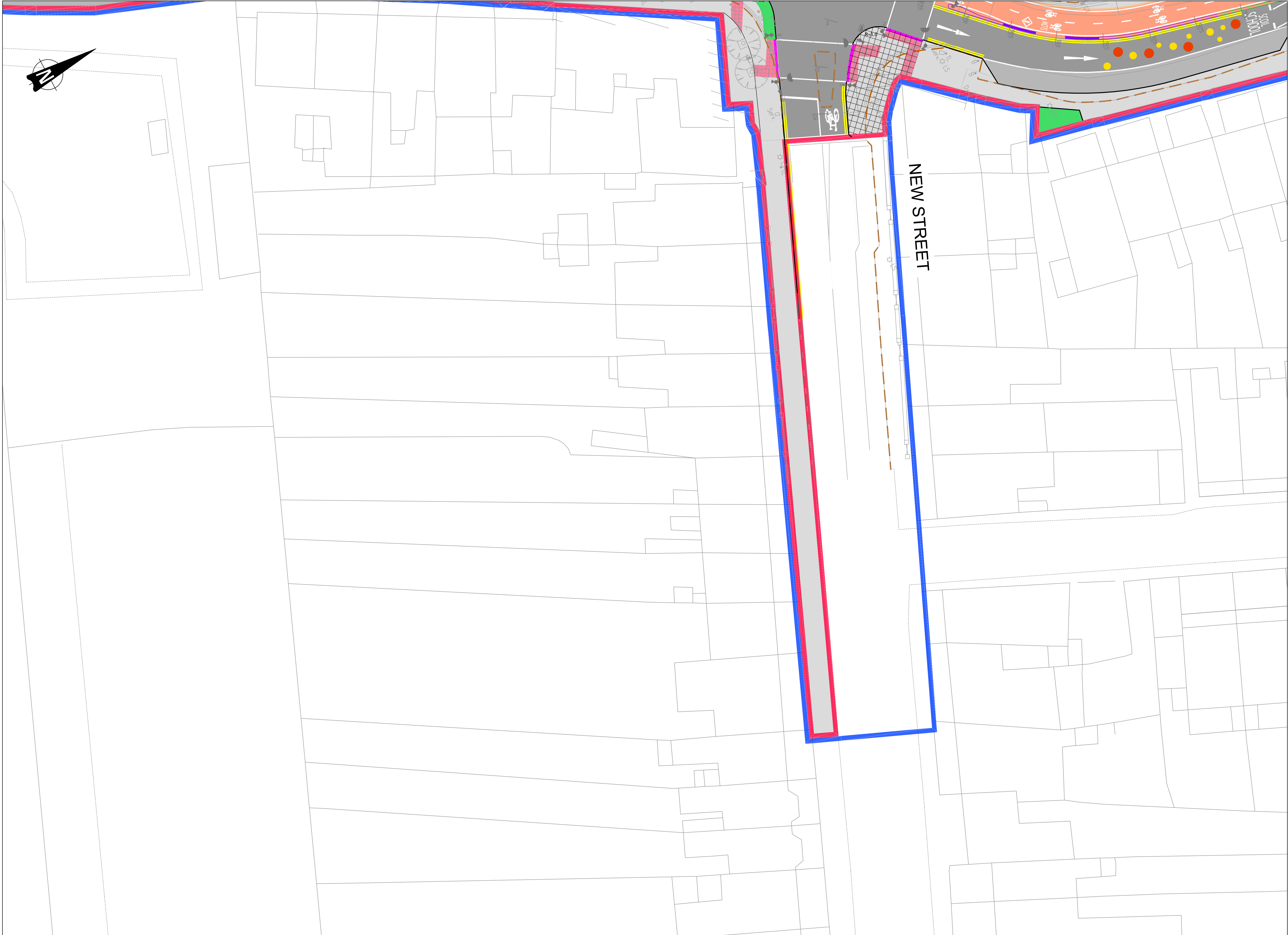
1:200 ROADS LAYOUT
