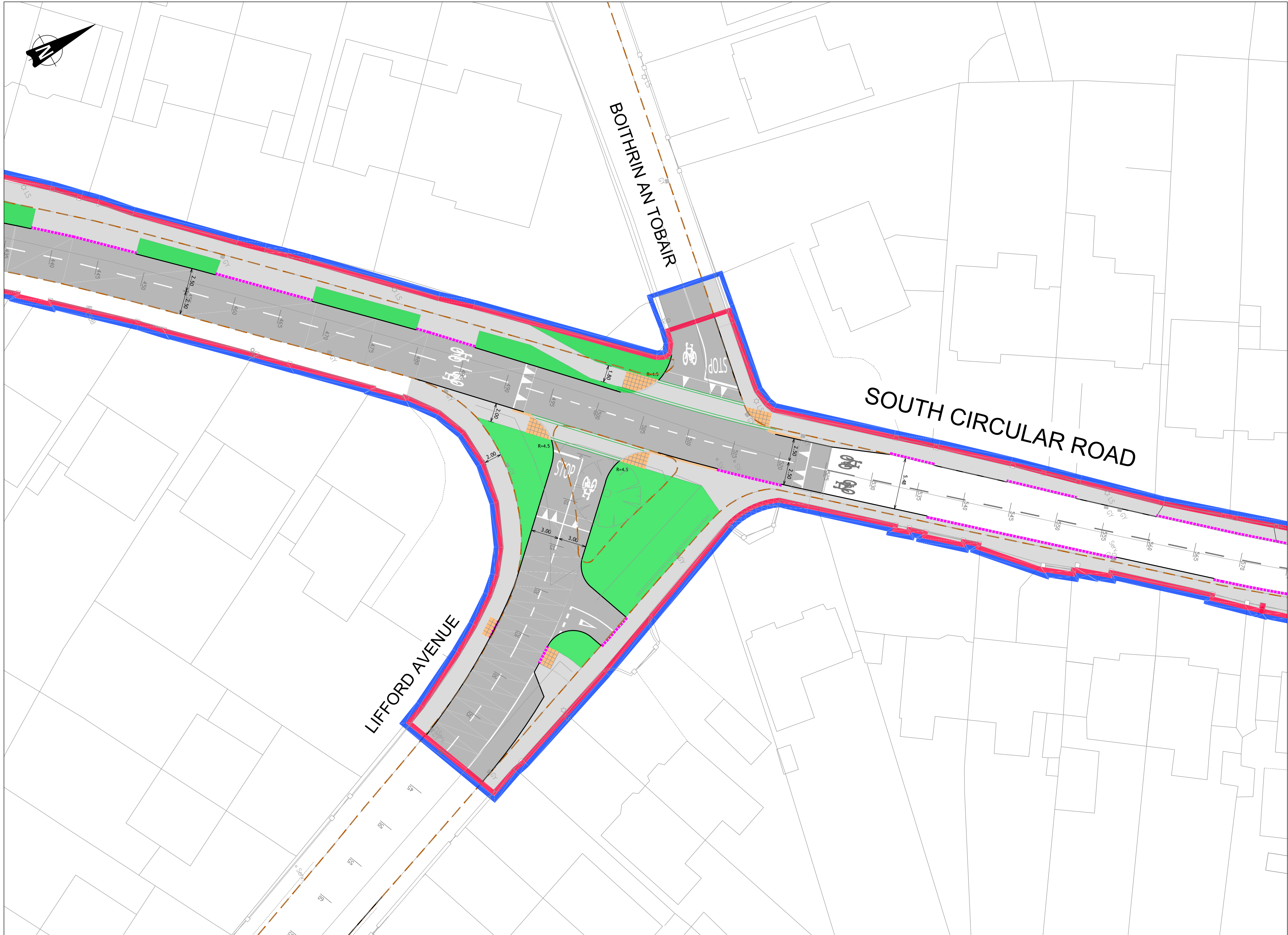
1:200 ROADS LAYOUT
