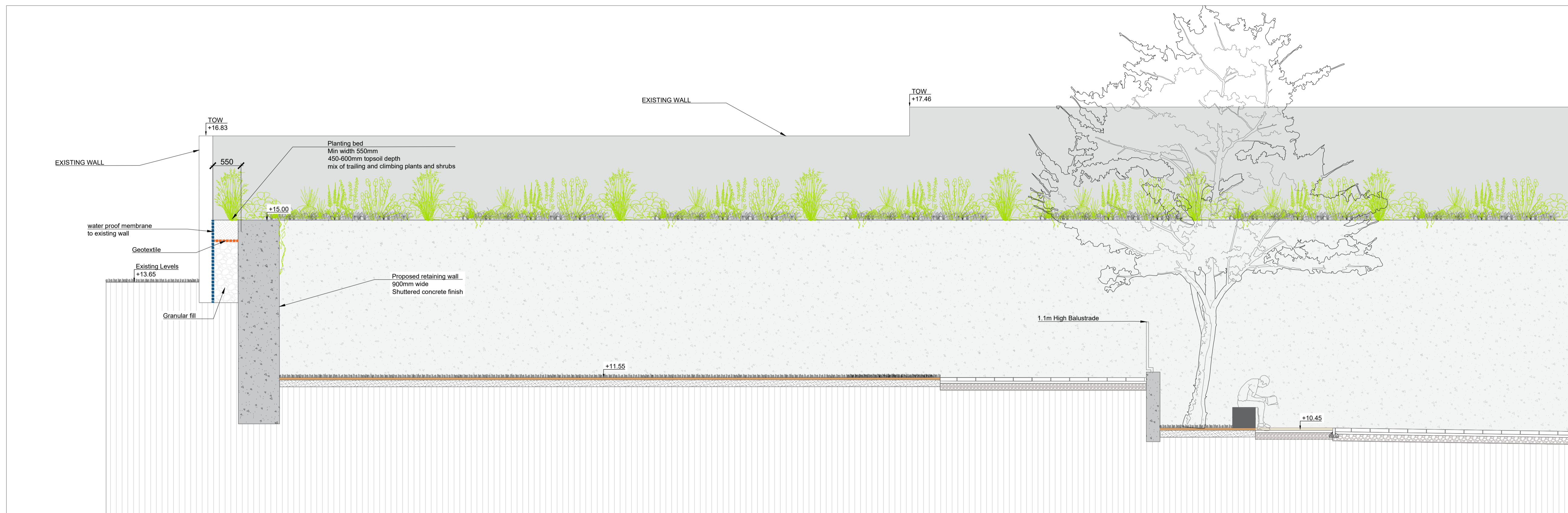
STONETOWN TERRACE NORTH BOUNDARY ELEVATION - SCALE 1:50 @A1 01 2010
