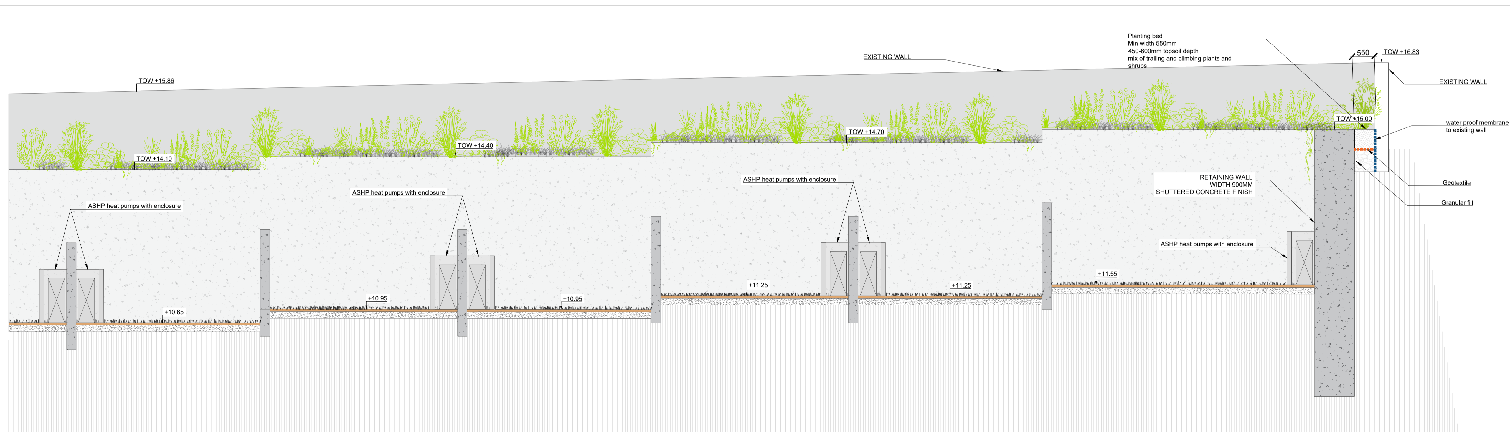
STONETOWN TERRACE WEST BOUNDARY ELEVATION - SCALE 1:50 @A1 02 2010
