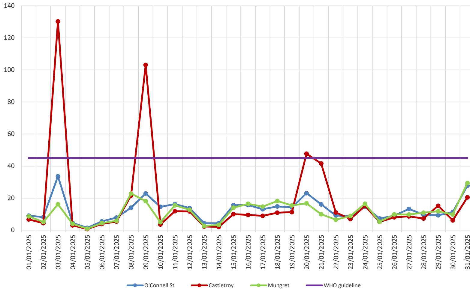
Particulate Matter < 10 microns (PM10) 24 hour mean ( \mu\text{g}/\text{m}^3 )
