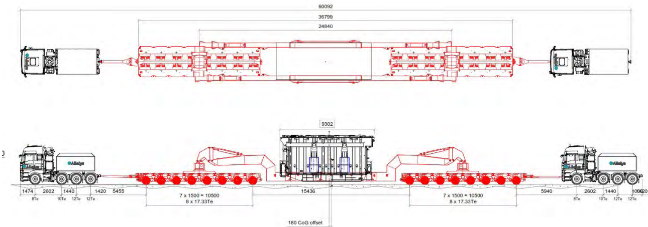
Figure 2 - schematic of 300T load
