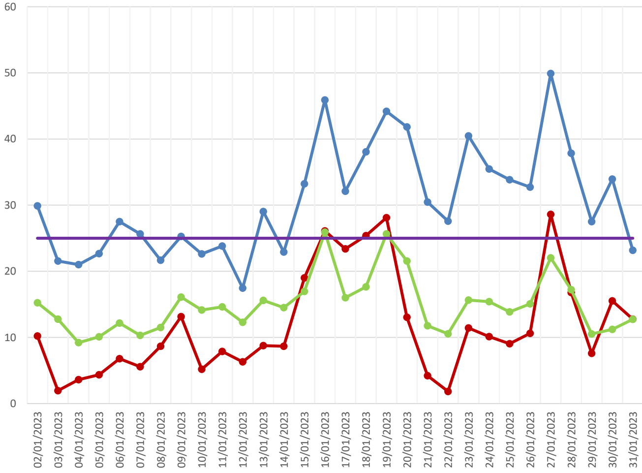
NO 2 - 24 hour mean (µg/m 3 )
