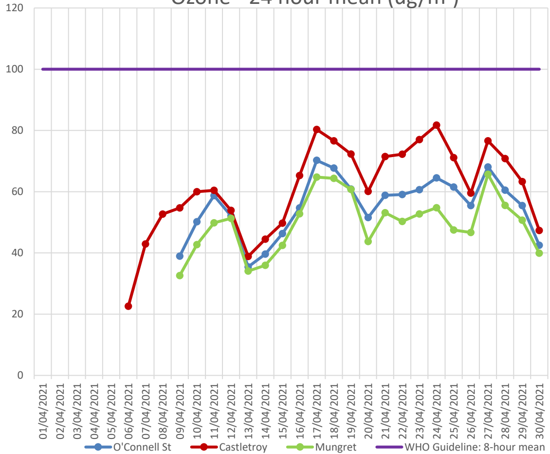
Ozone - 24 hour mean (ug/m 3 )
