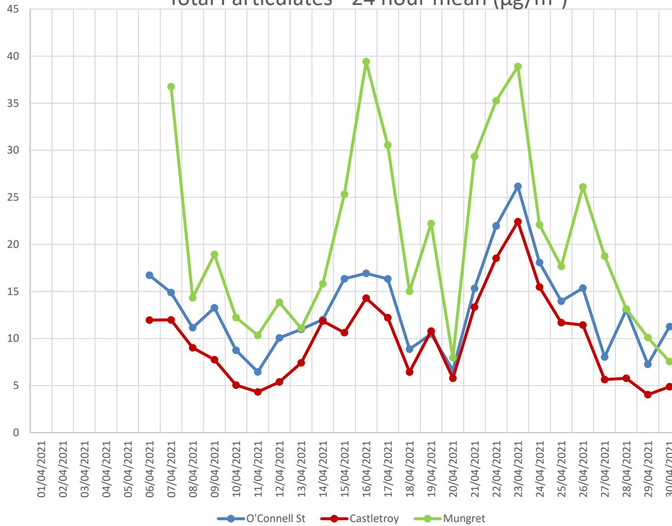
Total Particulates - 24 hour mean ( \mu\text{g}/\text{m}^3 )
