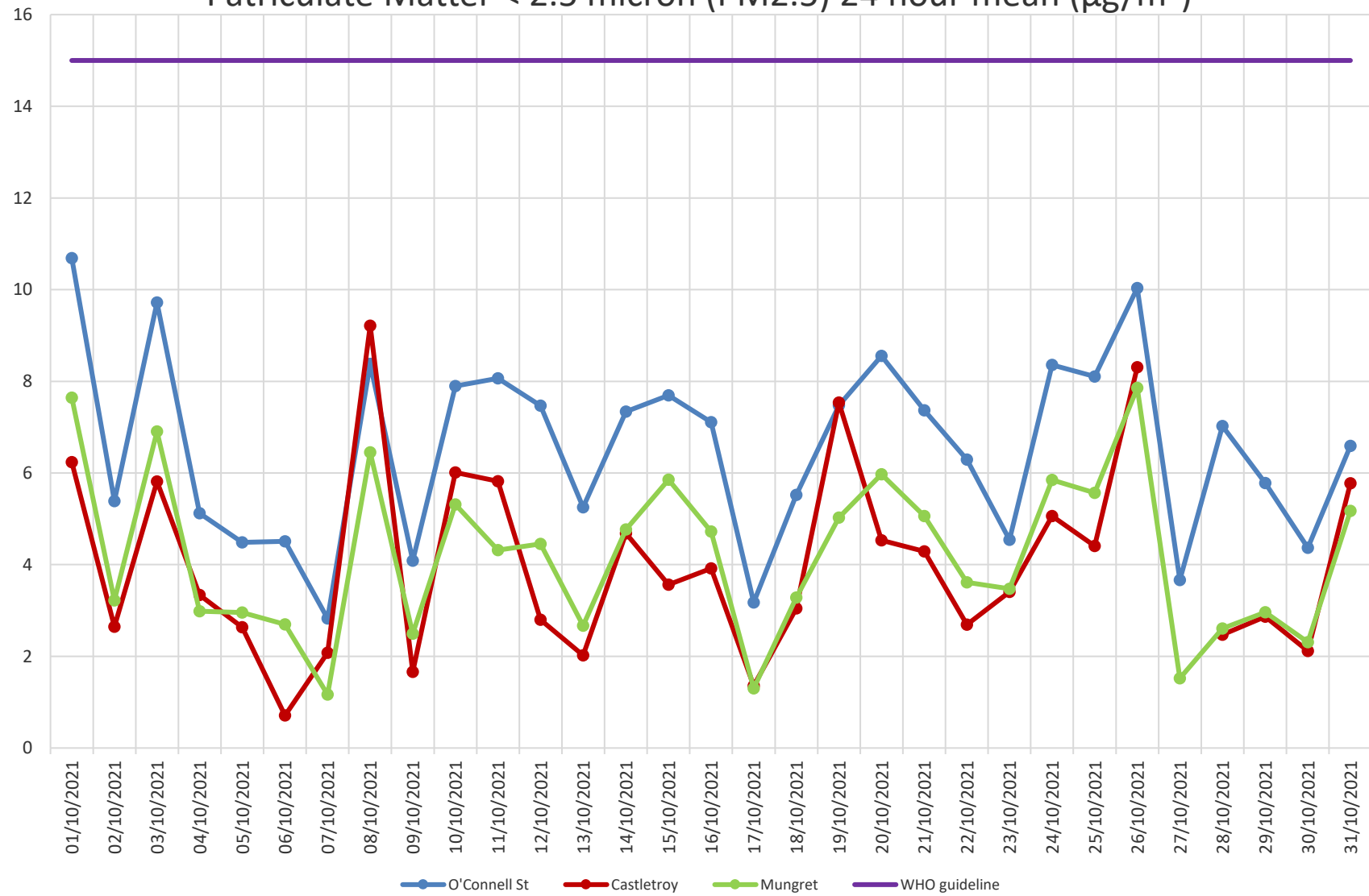
Particulate Matter < 2.5 micron (PM2.5) 24 hour mean ( \mu\text{g}/\text{m}^3 )
