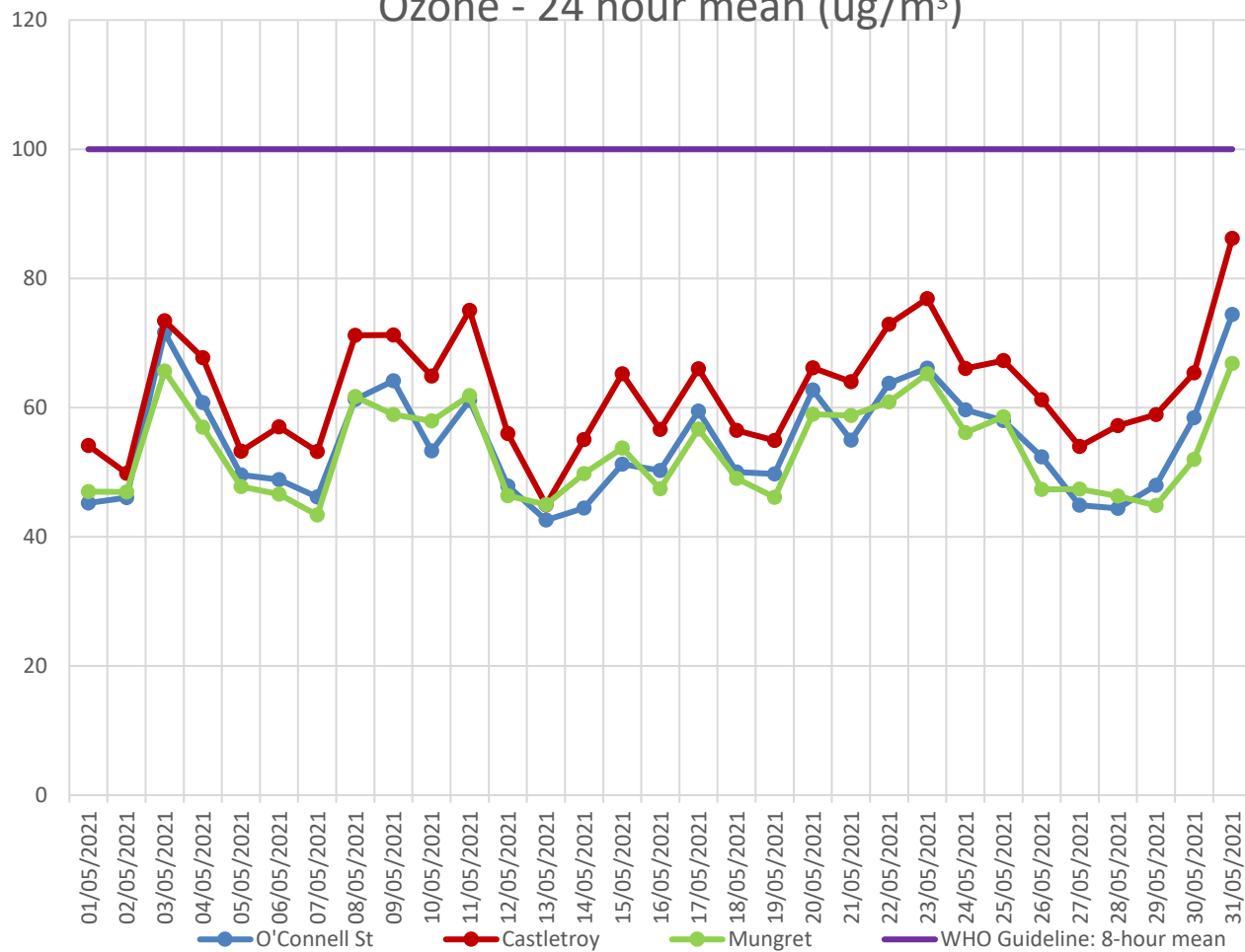
Ozone - 24 hour mean ( \mu\text{g}/\text{m}^3 )
