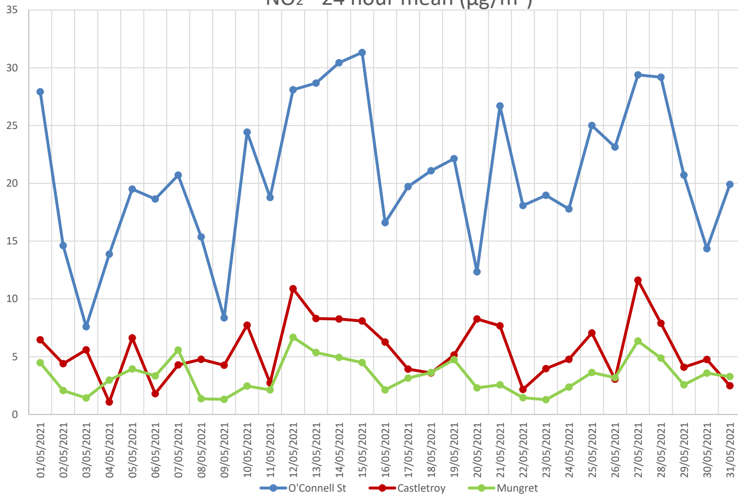
NO 2 - 24 hour mean (µg/m 3 )
