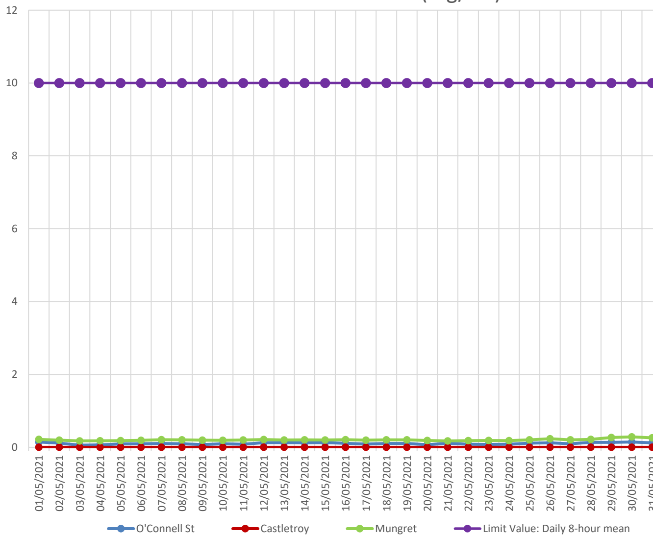
CO - 24 hour mean (mg/m 3 )
