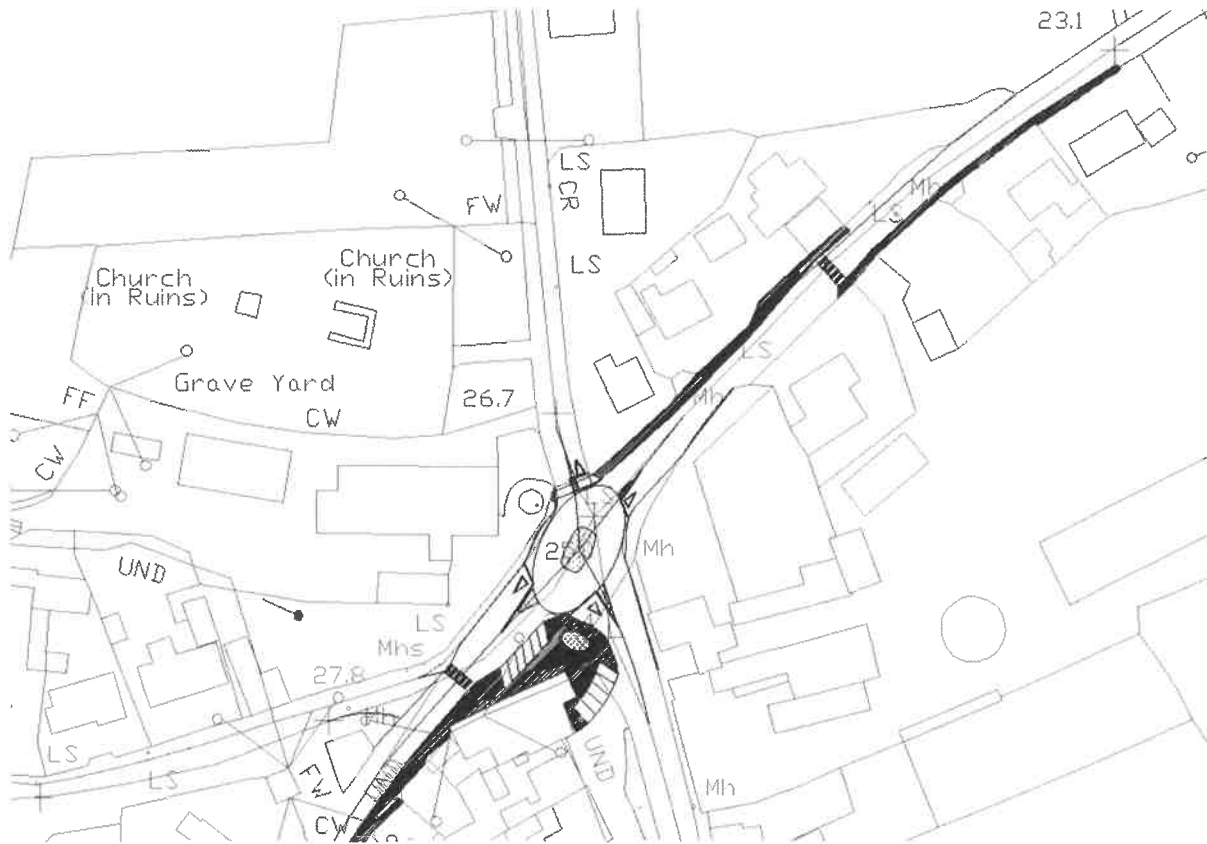
Shanagolden Traffic Calming
