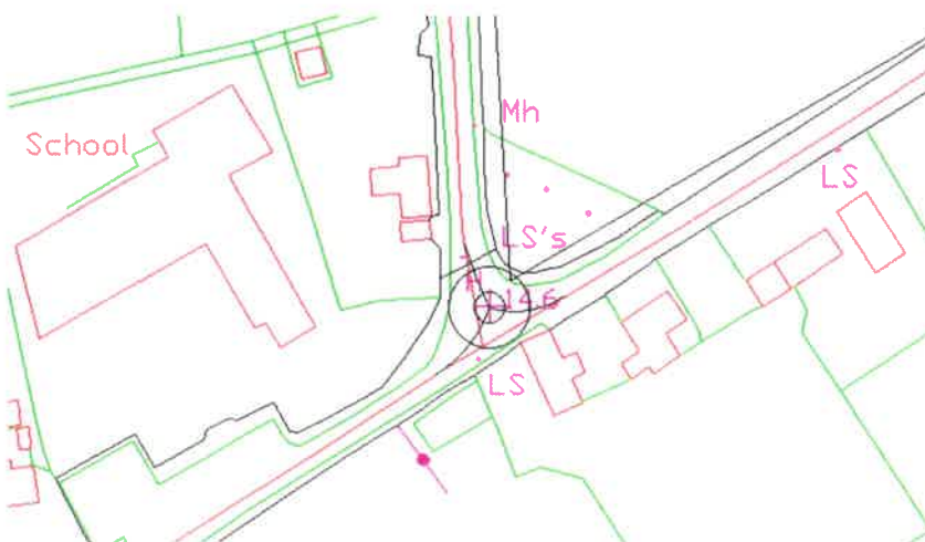
Preliminary Design of Proposed Mini Roundabout Pallaskenry
