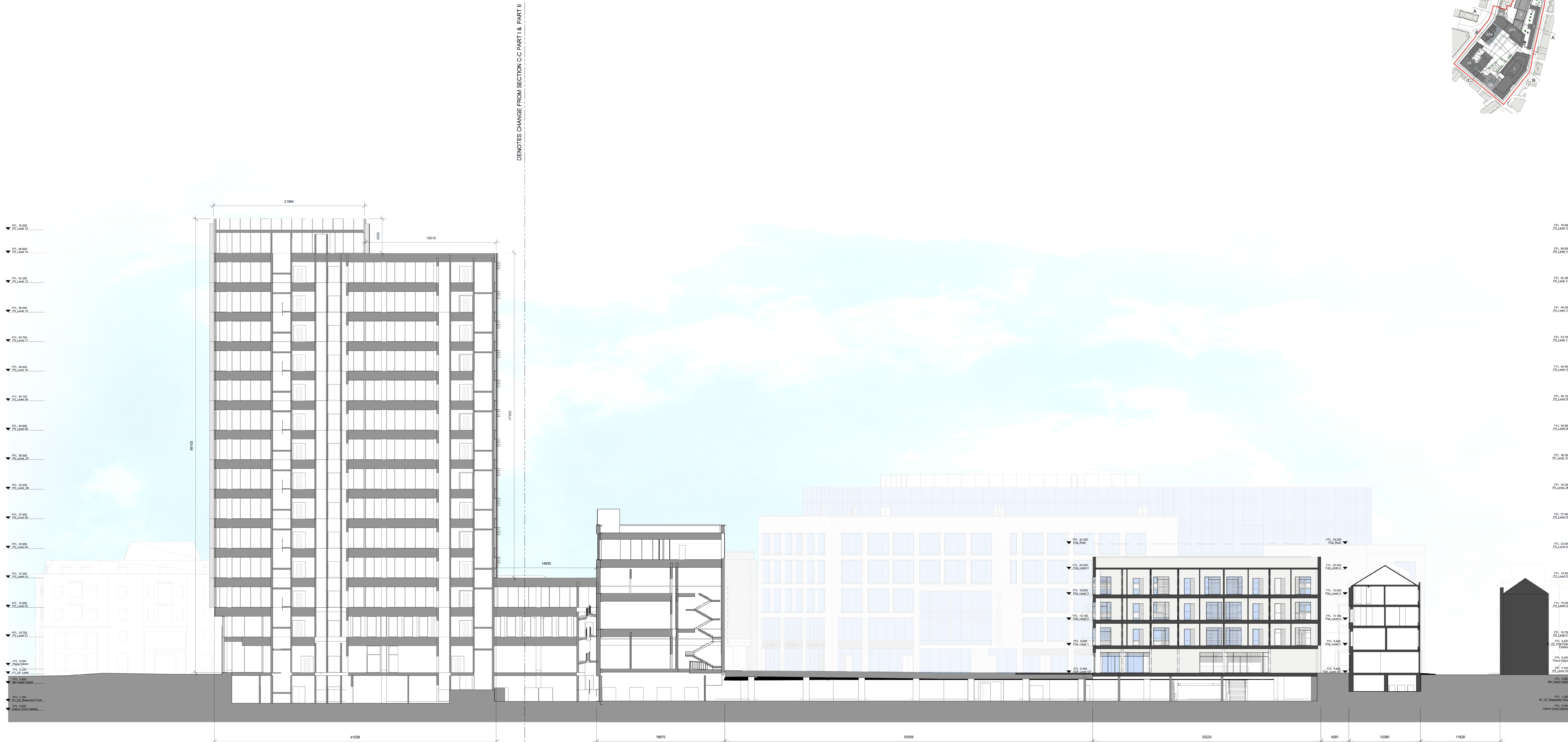
C-C Site Section C-C Part 1 SCALE: 1 : 200
