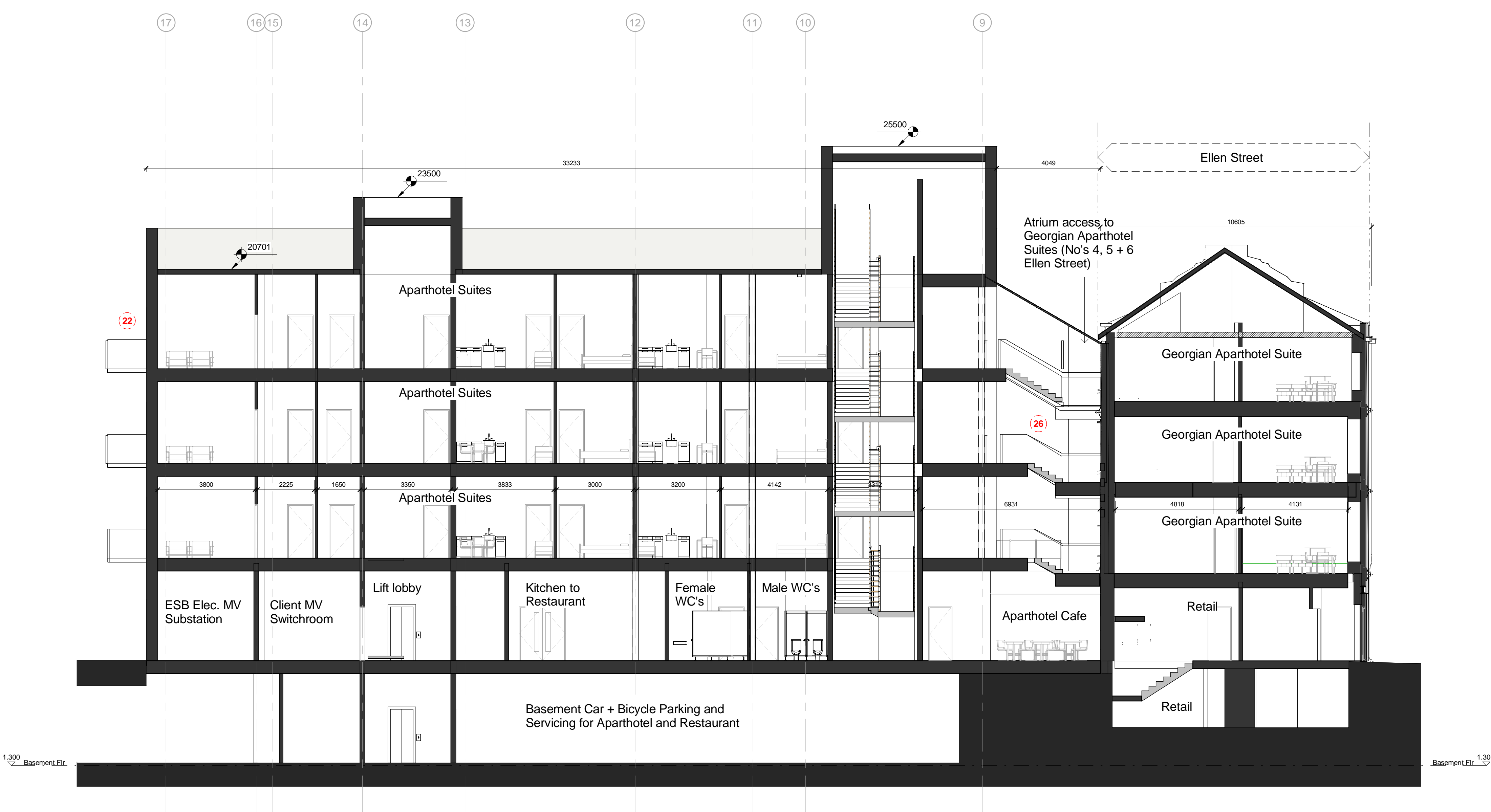
D-D | Section through No 4 Ellen Street + Aparthotel
