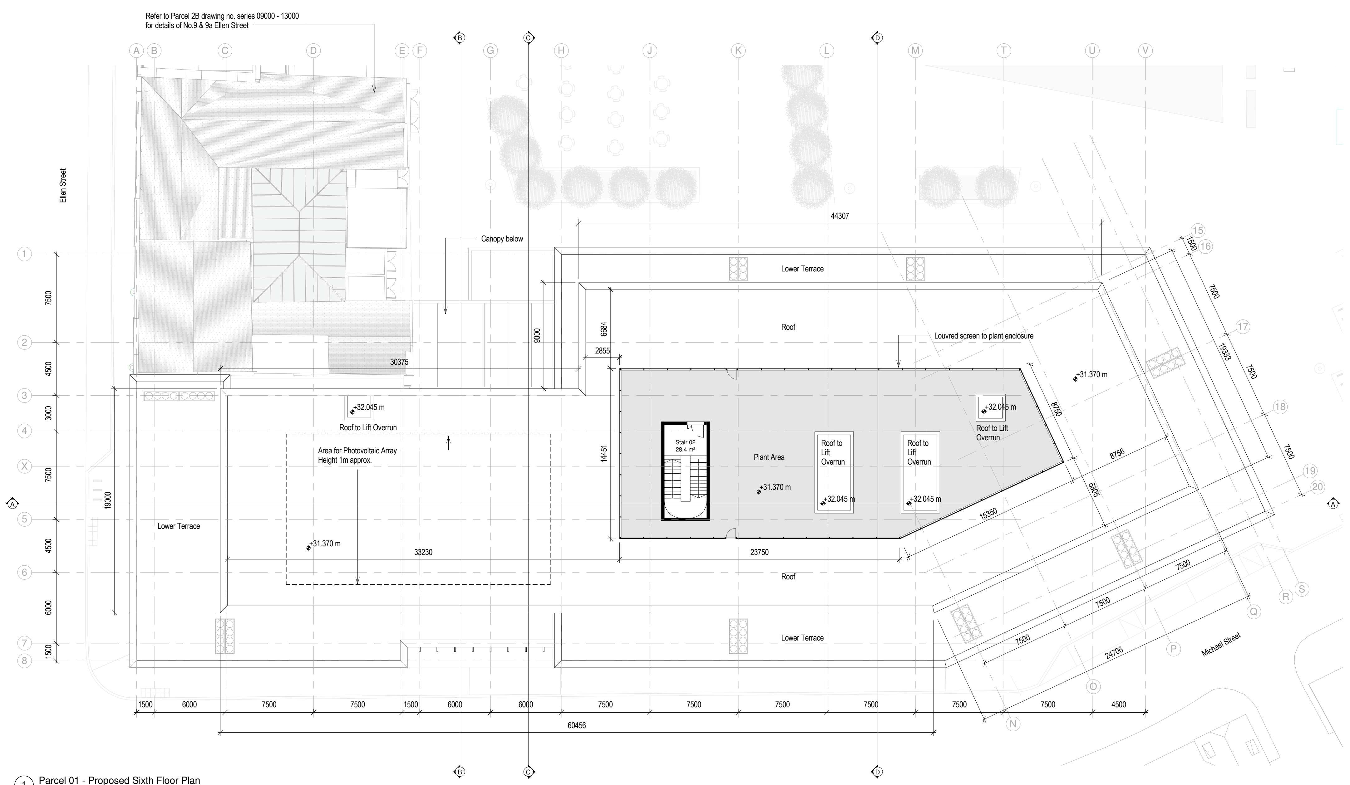
1 Parcel 01 - Proposed Sixth Floor Plan 1:200
