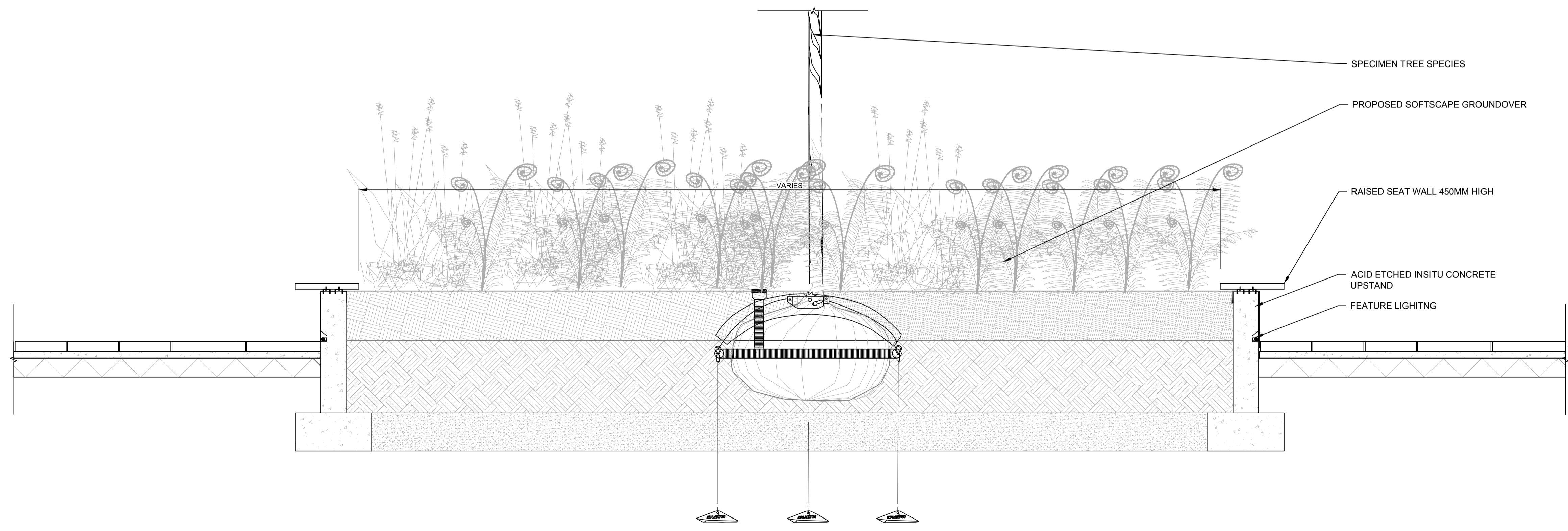
02 RAISED PLANTER ON GRADE 7003 Scale 1:20@A1
